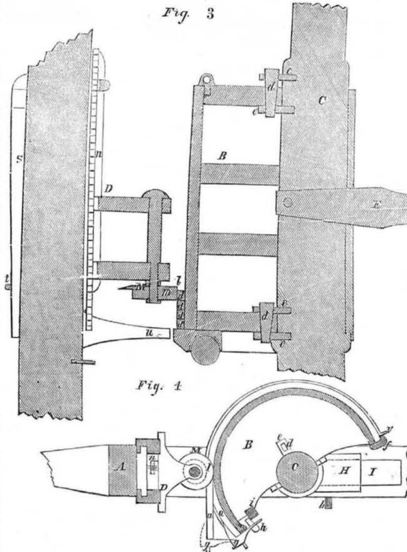
M, arranged and operating as hereinafter described. Secondly, in the manner of perfectly bending the last end of each felly and securing it when completely bent upon the mold, viz., by the combined action of the bending wheel, M,
