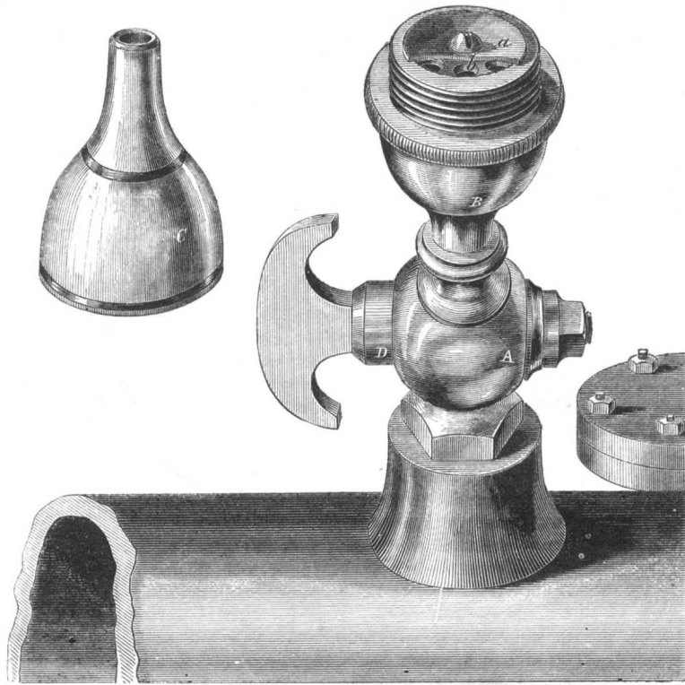
SHAW'S AIR VALVE FOR PUMPS.
