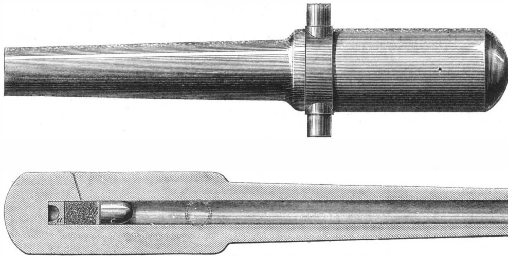
DAY'S ELASTIC BREECH CANNON AND INDIA-RUBBER SABOT.
