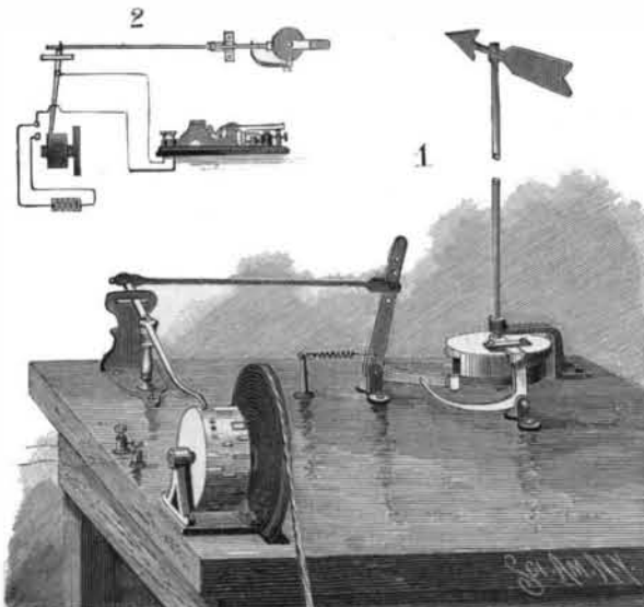
DAVIS AND CHRISTY'S SIGNAL TRANSMITTER.
