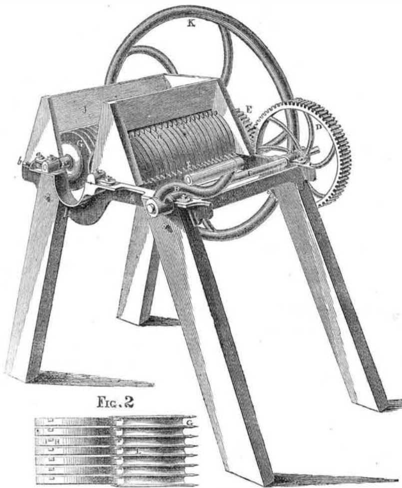
STRAW CUTTER.—Fig. 1.
