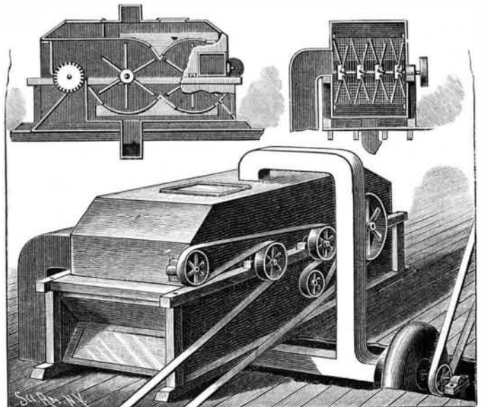
WILSON'S SEED COTTON CLEANER.
