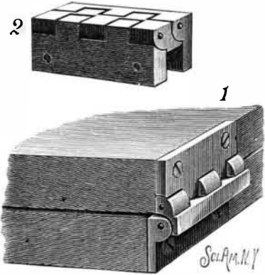
LARIMER'S HINGE.
