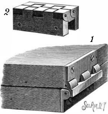
LARIMER'S HINGE.
