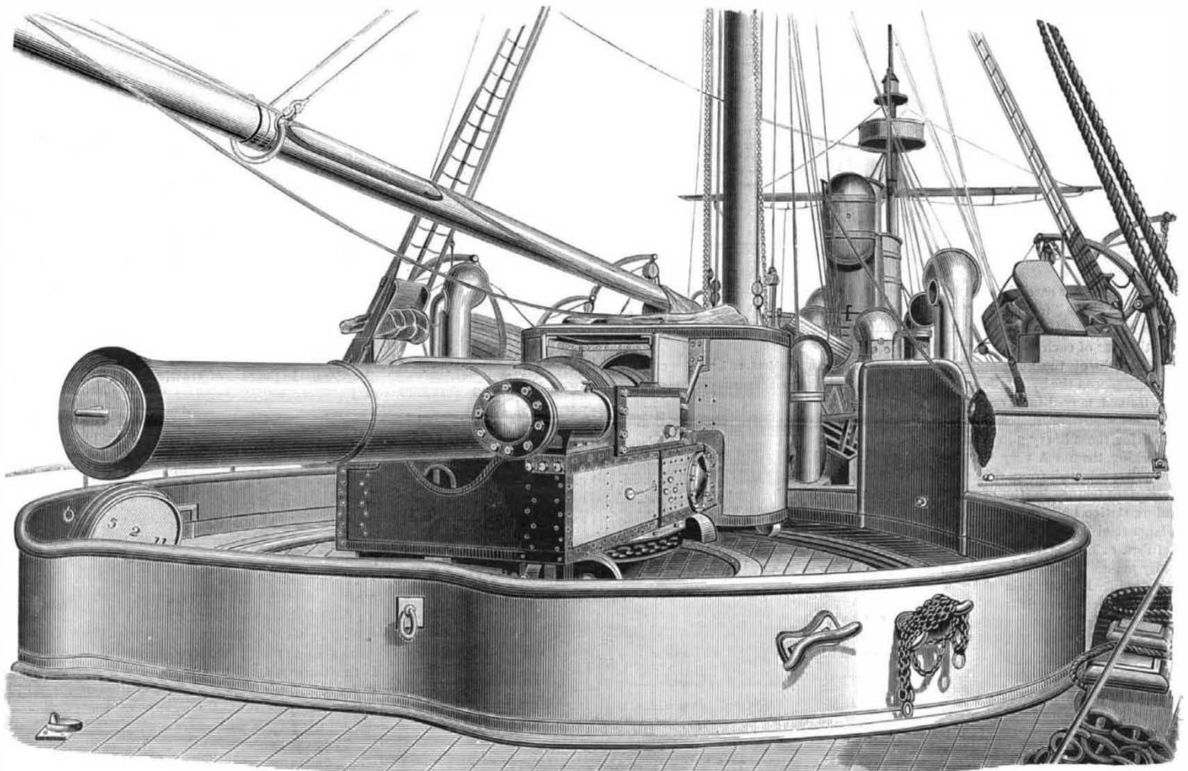
THE GUNS OF THE ESMERALDA.—TWENTY-FIVE TON STERN CHASER.
