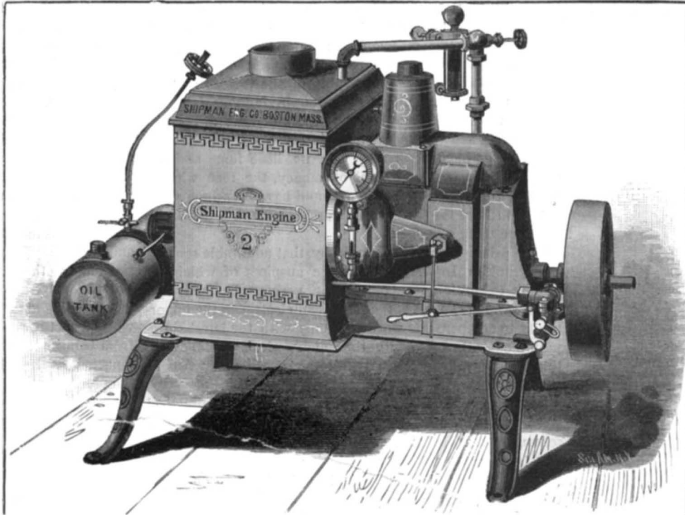
NEW SHIPMAN ENGINE NO. 2.
