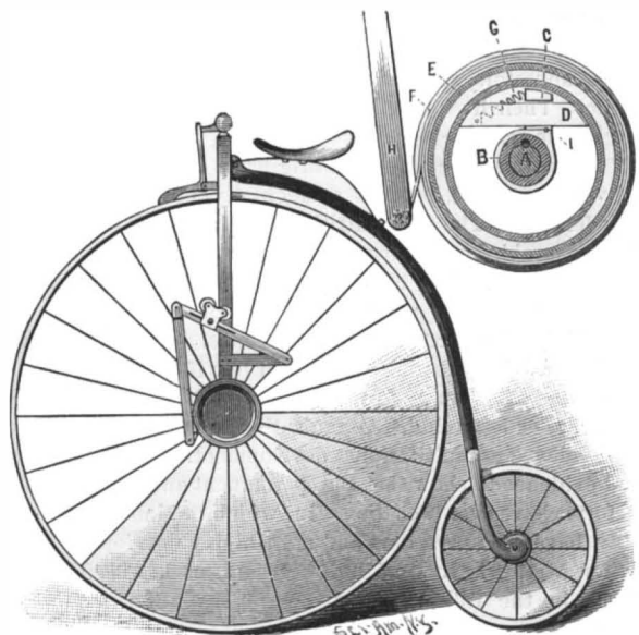
DE BEAULIEU'S DRIVING MECHANISM FOR VELOCIPEDES.
