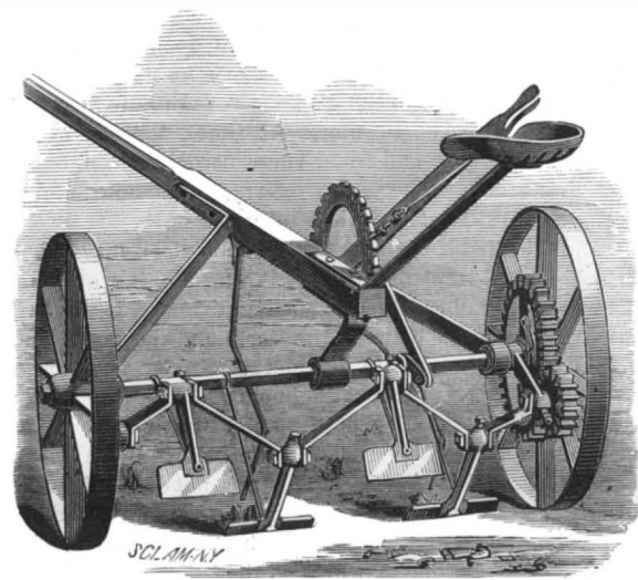
GILLET'S SULKY CORNSTALK CUTTER.
