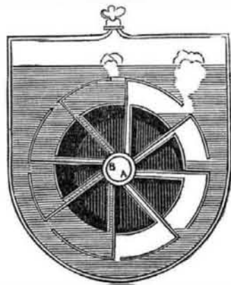
STEAM WHEEL. FIG. 51.
