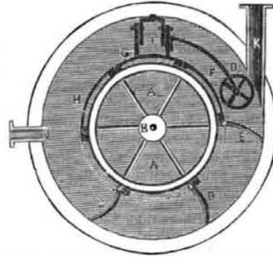
FOREMAN'S ROTARY ENGINE. FIG. 49.
