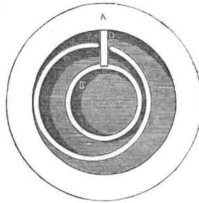
TROTTER'S ROTARY ENGINE. FIG. 24.
