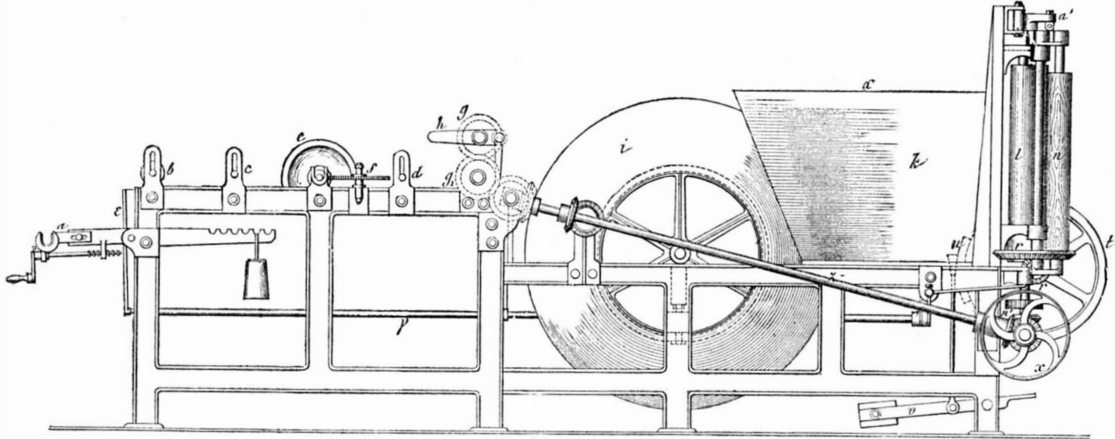
CLOTH-FOLDING MACHINE.—Fig. 1.
