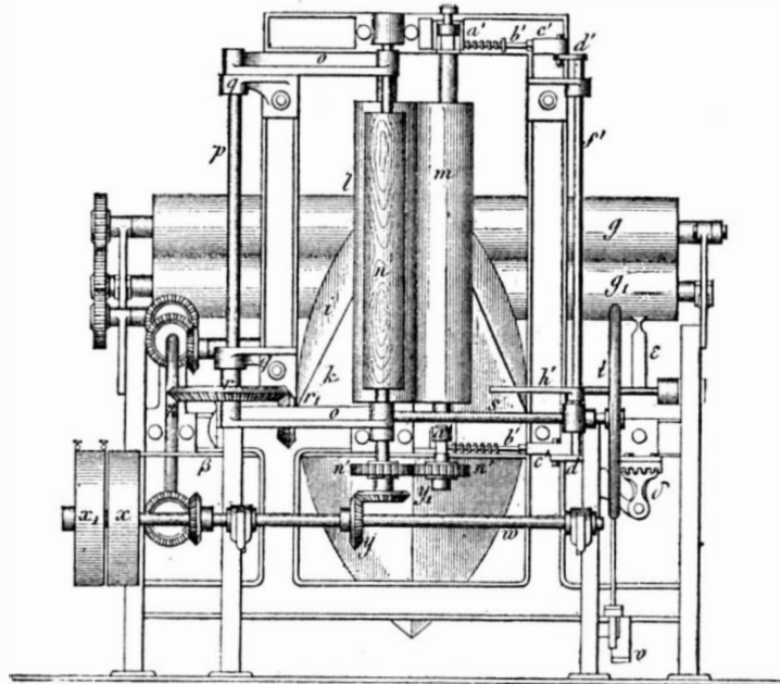
CLOTH FOLDING MACHINE.—Fig. 2.
