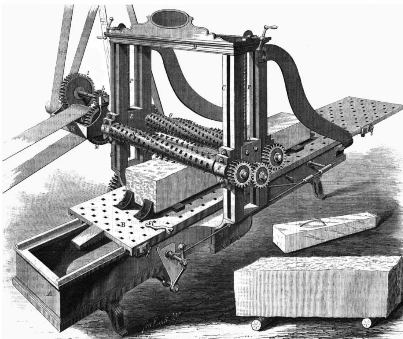
ANDERSON'S STONE DRESSING MACHINE.
