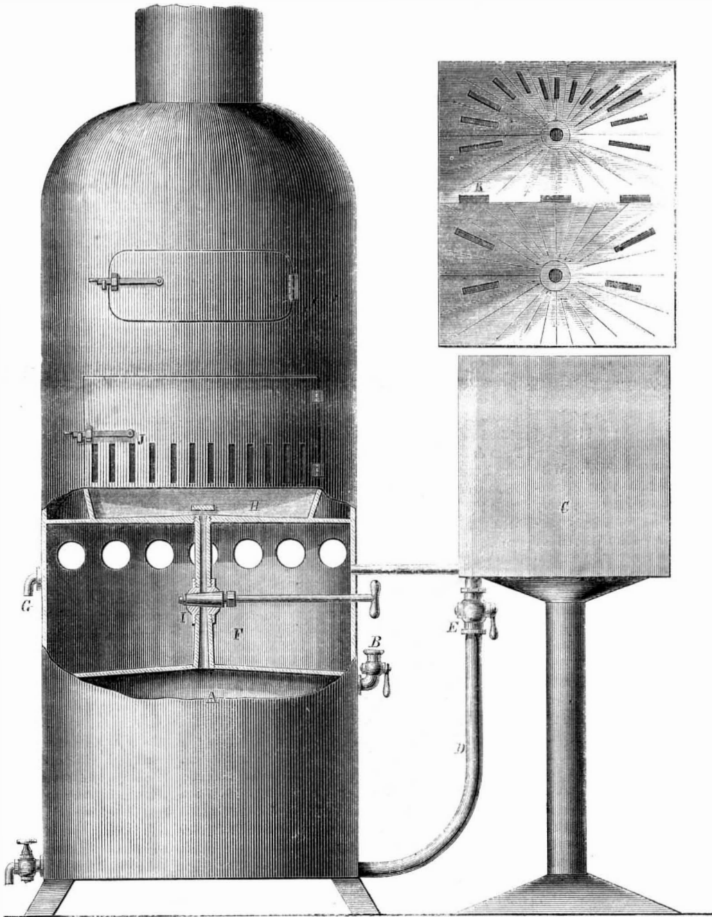
M'KINNEY'S APPARATUS FOR BURNING PETROLEUM.
