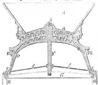
Adjustable Grinding Iron Mill.
